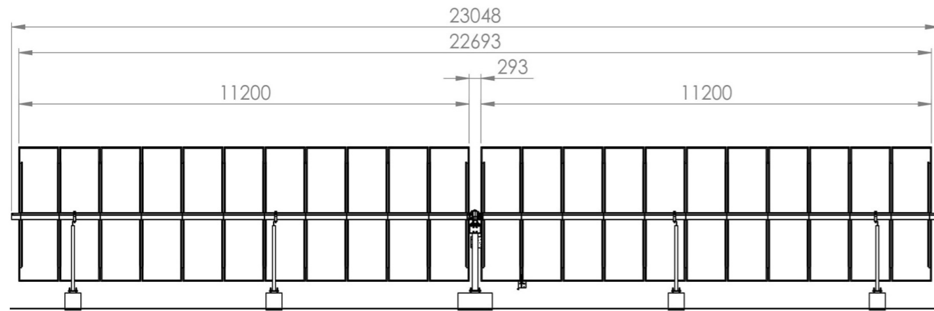
DEGER S100-CF-DR With Concrete Foundation (1)
