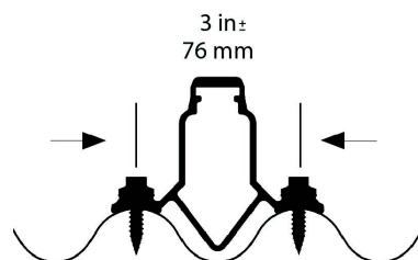
Figure 6: Corrugated Roof Min and Max Rib Span
