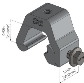
S-5-K Grip™
