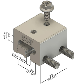
S-5-T™
