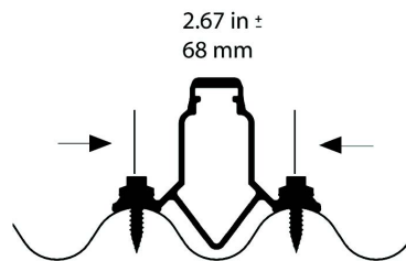
Figure 6: Corrugated Roof Min and Max Rib Span
