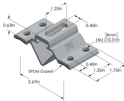
CorruBracket™ 100T
