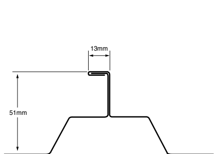
51mm Trap Single Fold S-5-S, S-5-S Mini
