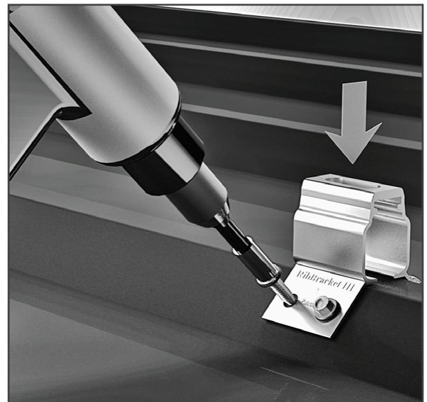
Step 3: Install fasteners
