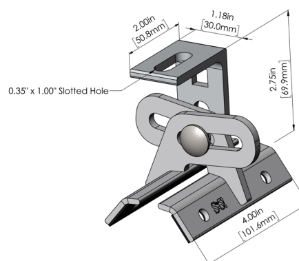
ProteaBracket™
