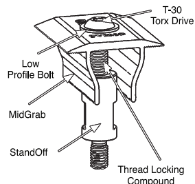
MidGrab/StandOff Assembly
