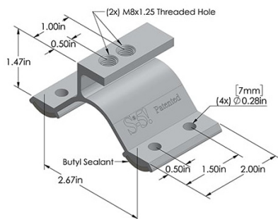
CorruBracket™
