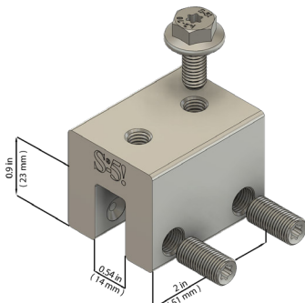
S-5-S™
