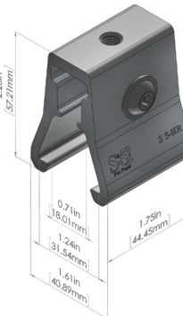
S-5-HR™
