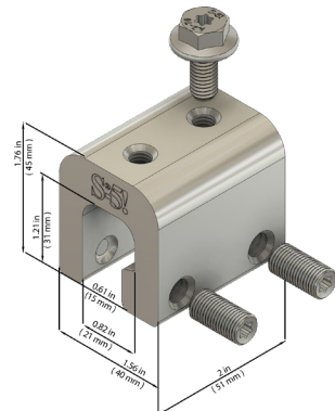
S-5-MX™
