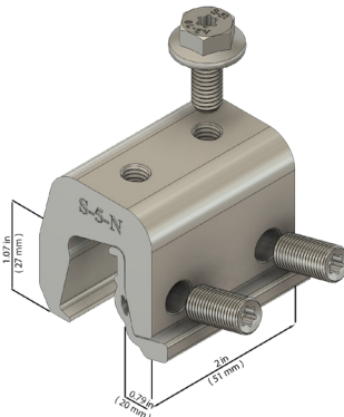
S-5-N™
