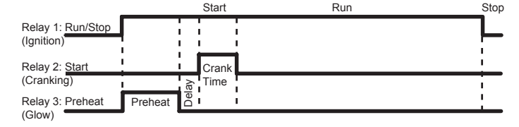
RunMode Timing Diagram for Gen Types 7, 8, and 14
