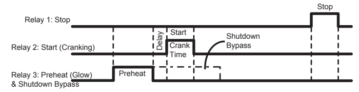
PulseStop Mode Timing Diagram for Gen Type 13
